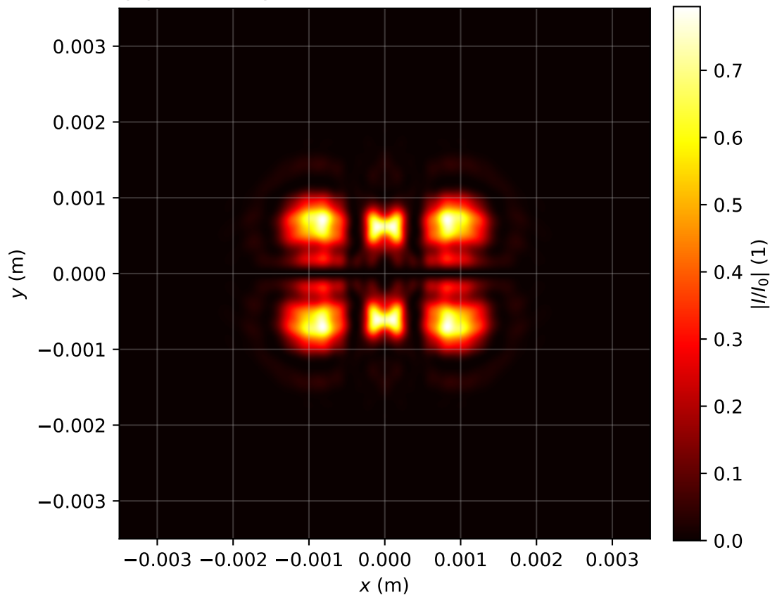
Intensity profile I(x, y, z = 1.194)/I_0 , P_{in}=7.0P_{cr} , artificial time
